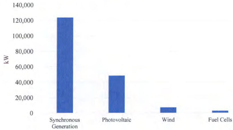
Figure 19: PJM Distributed Generation in PHI's Jurisdictions (Active)
